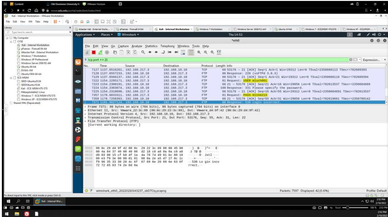
Figure 11 Internal Kali VM - TCP port 21 display filter demonstration II
