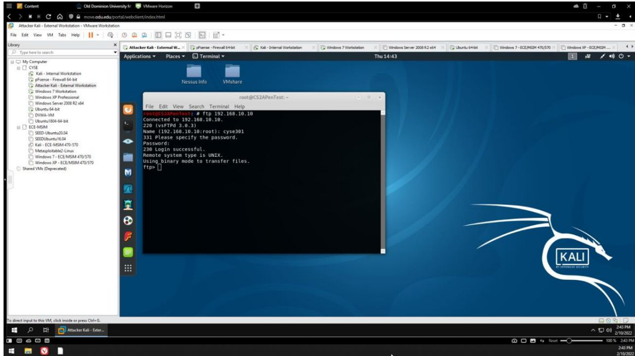
Figure 9 External Kali VM - Connecting to Ubuntu VM FTP server demonstration
