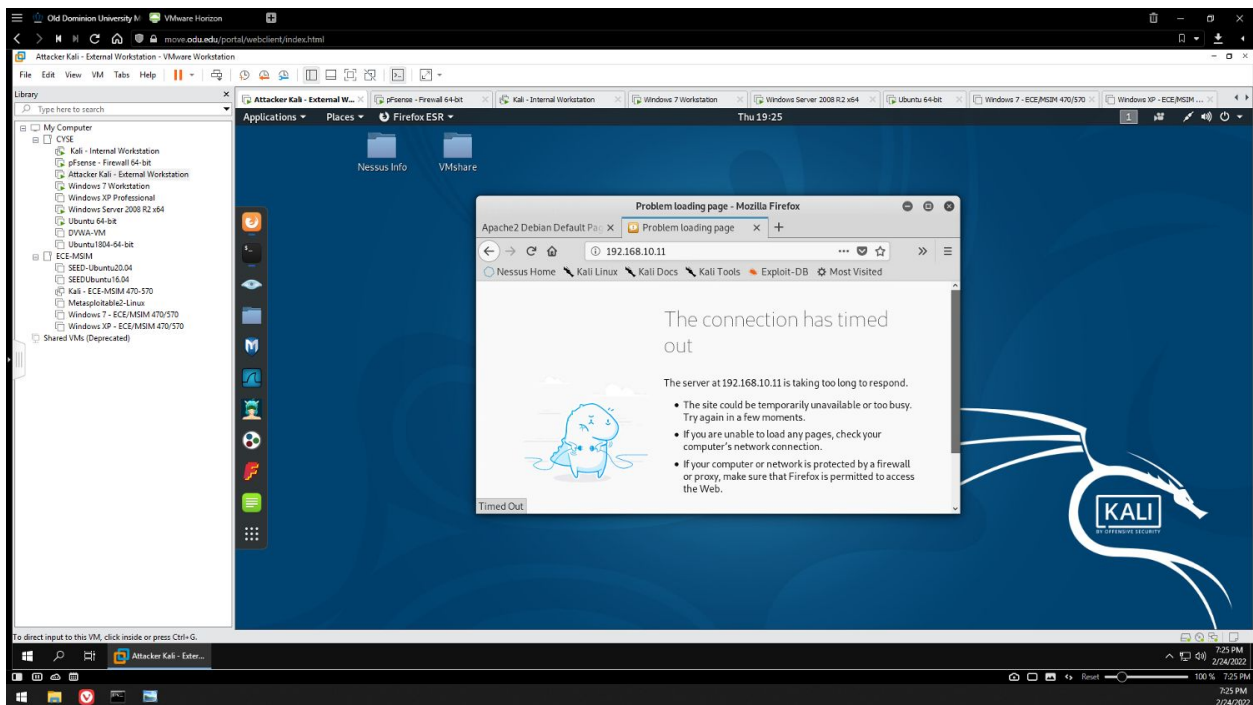
Figure 5 - Firewall ruleset demonstration: External Kali VM unable to connect to WS 2008 VM via HTTP
