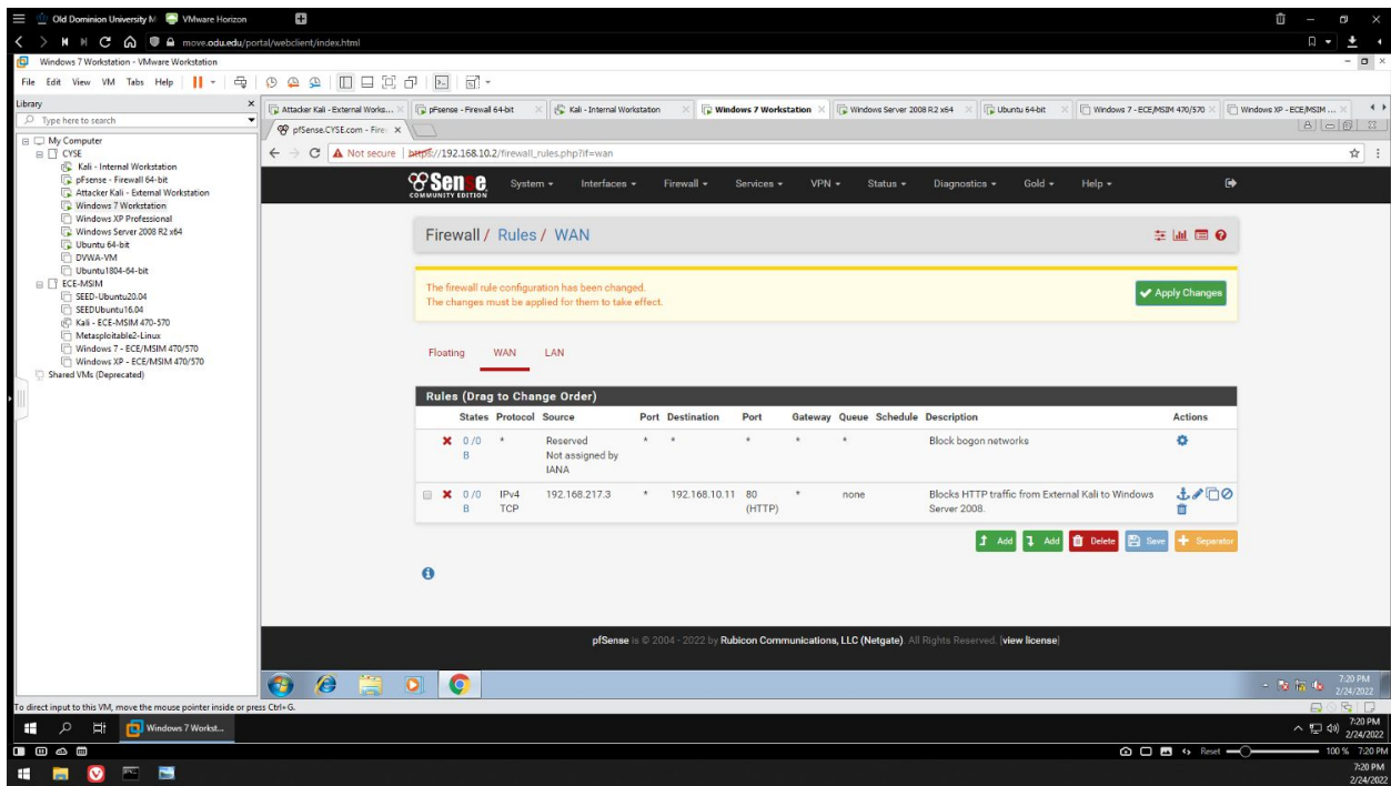
Figure 4 - Applying ruleset to block HTTP connection from External Kali VM to WS 2008 VM
