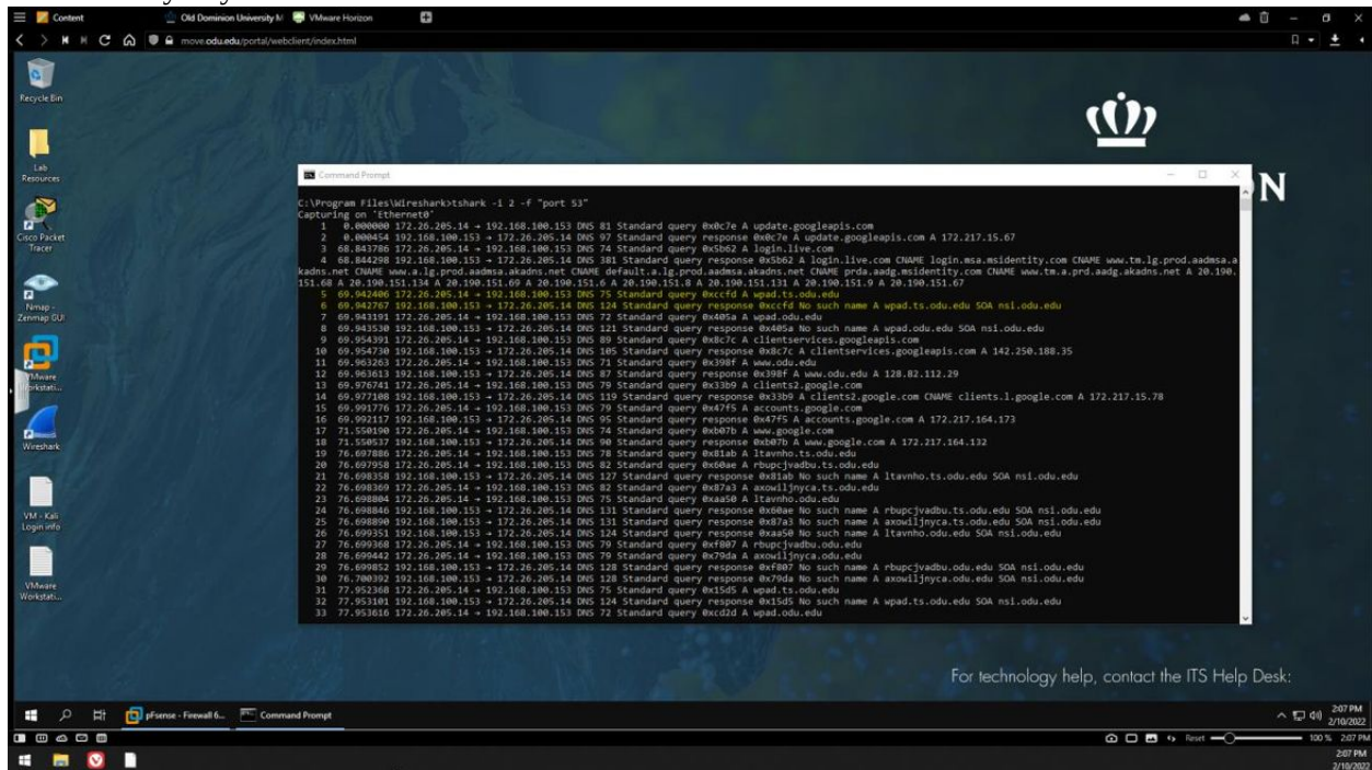
Figure 3 tShark w/ "port 53" capture filter active & DNS query, response packets
