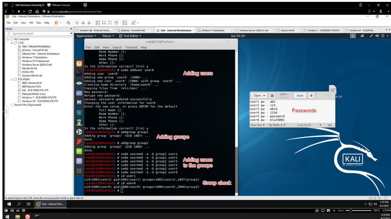
Figure 1 - Creating users and groups on Internal Kali
