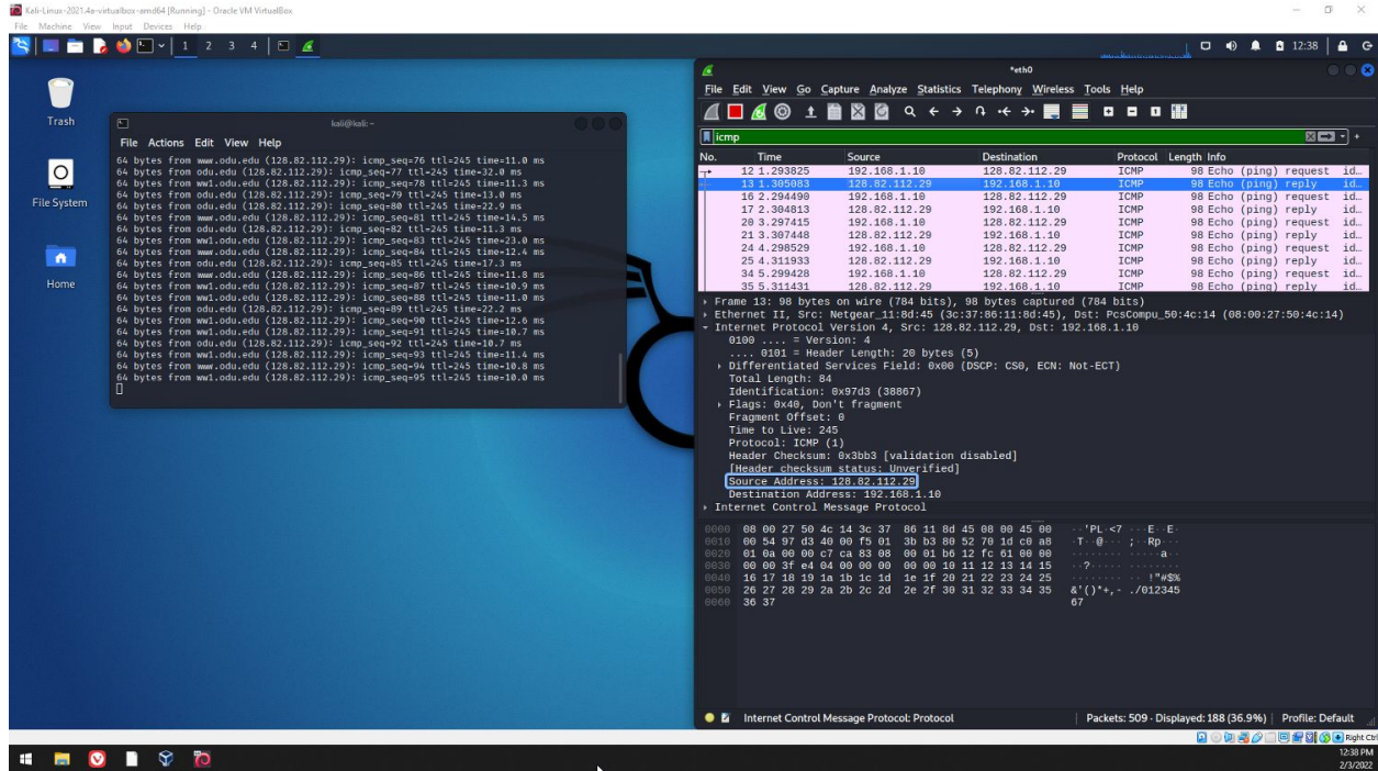
Figure 9 ICMP (ping) packets from www.odu.edu
