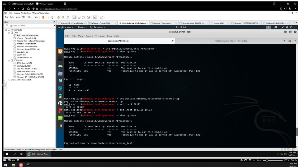
Figure 12 - Setting up the “bypassuac” exploit
