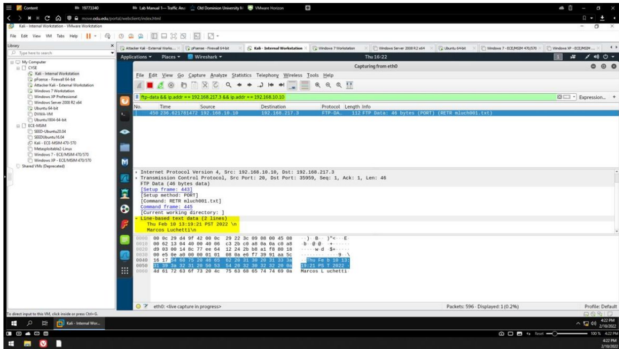
Figure 14 Internal Kali VM - Wireshark FTP-DATA display filter demonstration
