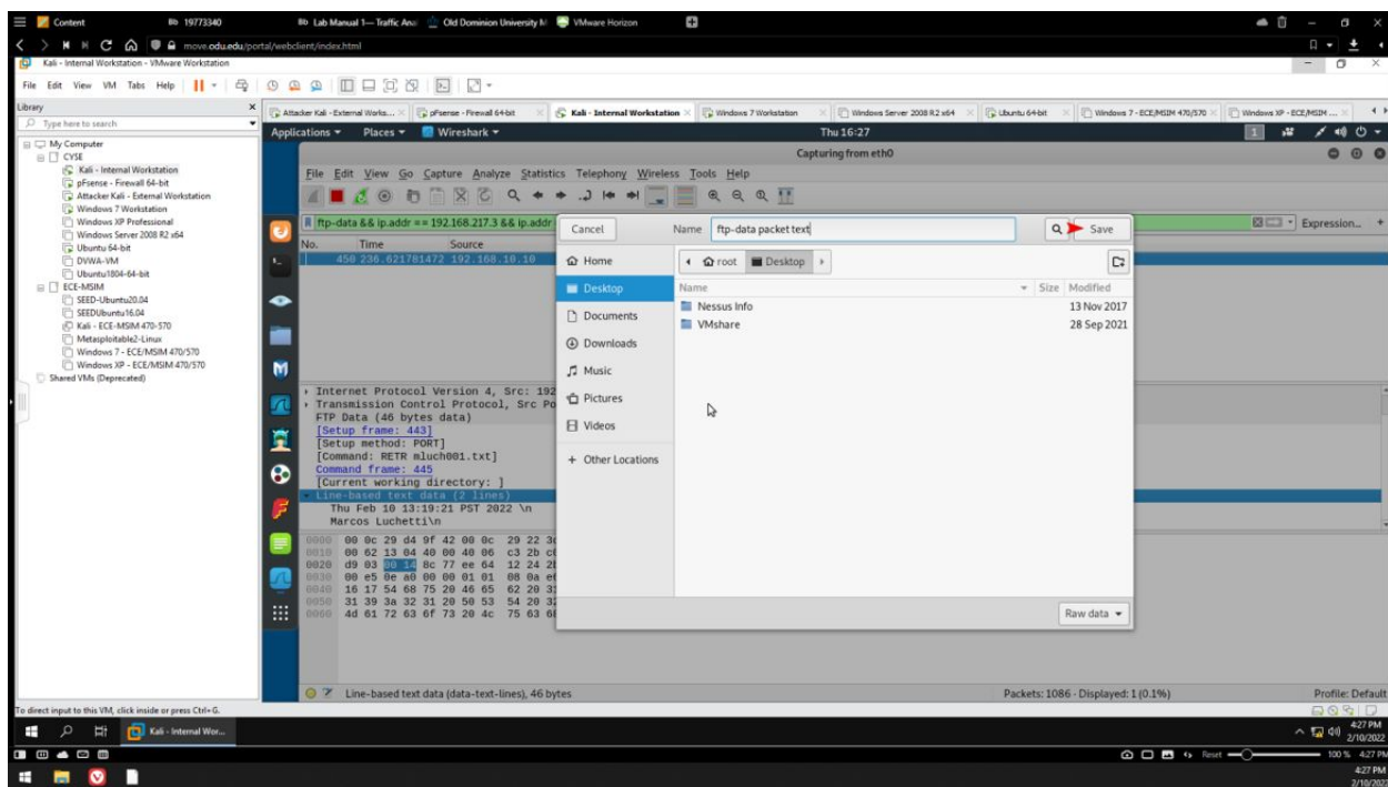
Figure 16 Internal Kali VM - Exporting packet data from Wireshark II
