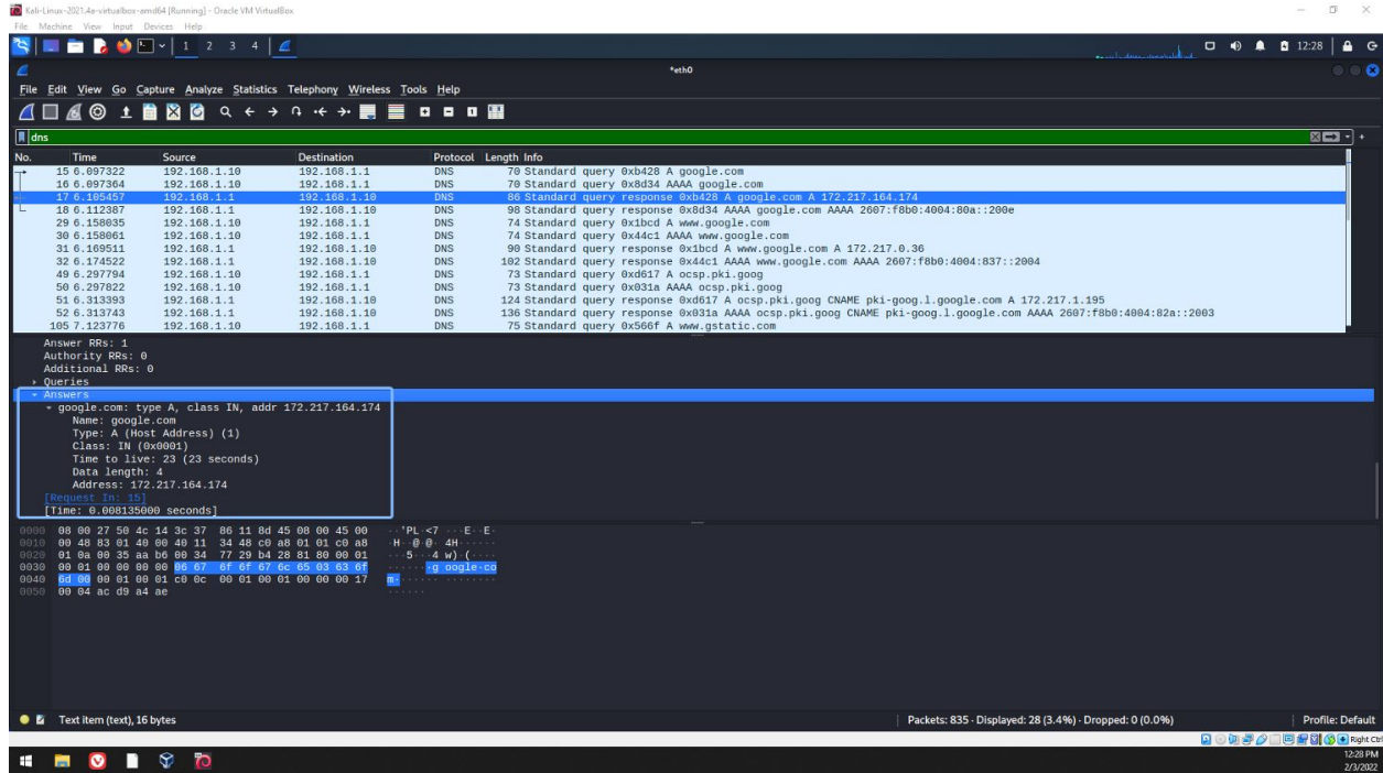
Figure 6 Query answers for first pair
