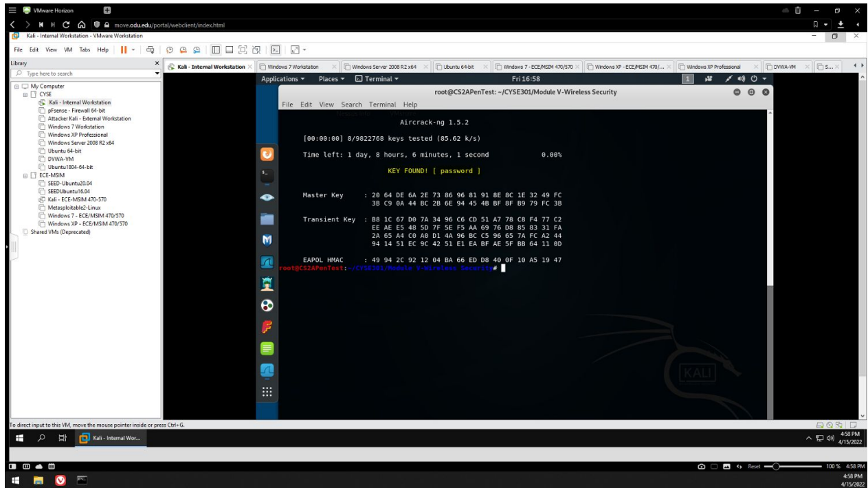
Figure 9 - lab4wpa2.cap key found
