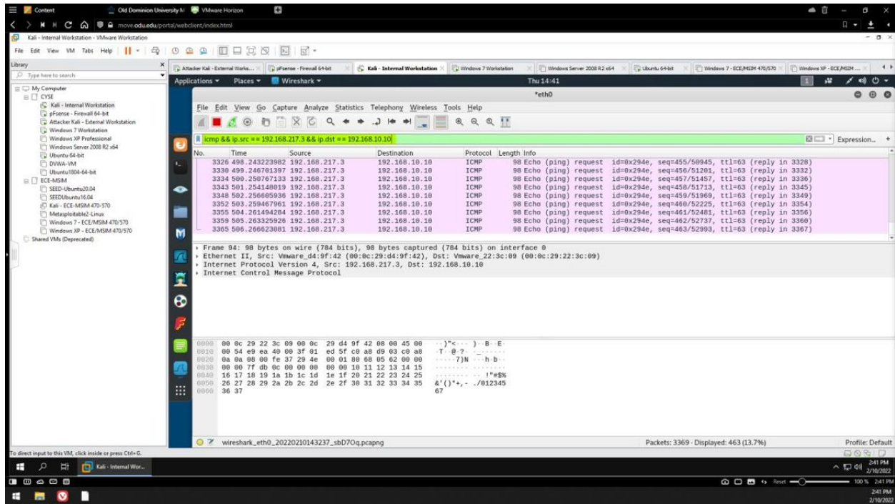
Figure 8 Display filter demonstration in Wireshark on Internal Kali VM
