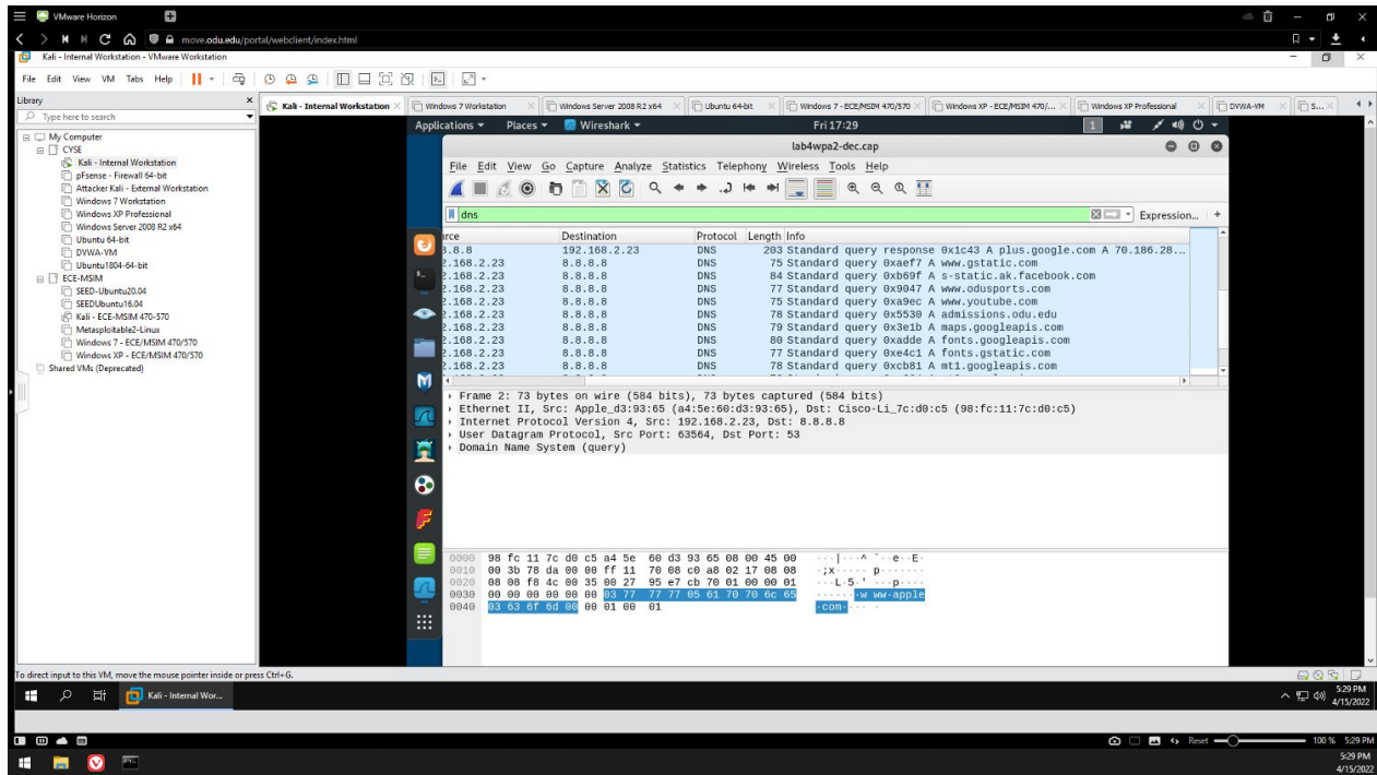
Figure 12 - lab4pa2-dec.cap DNS queries
