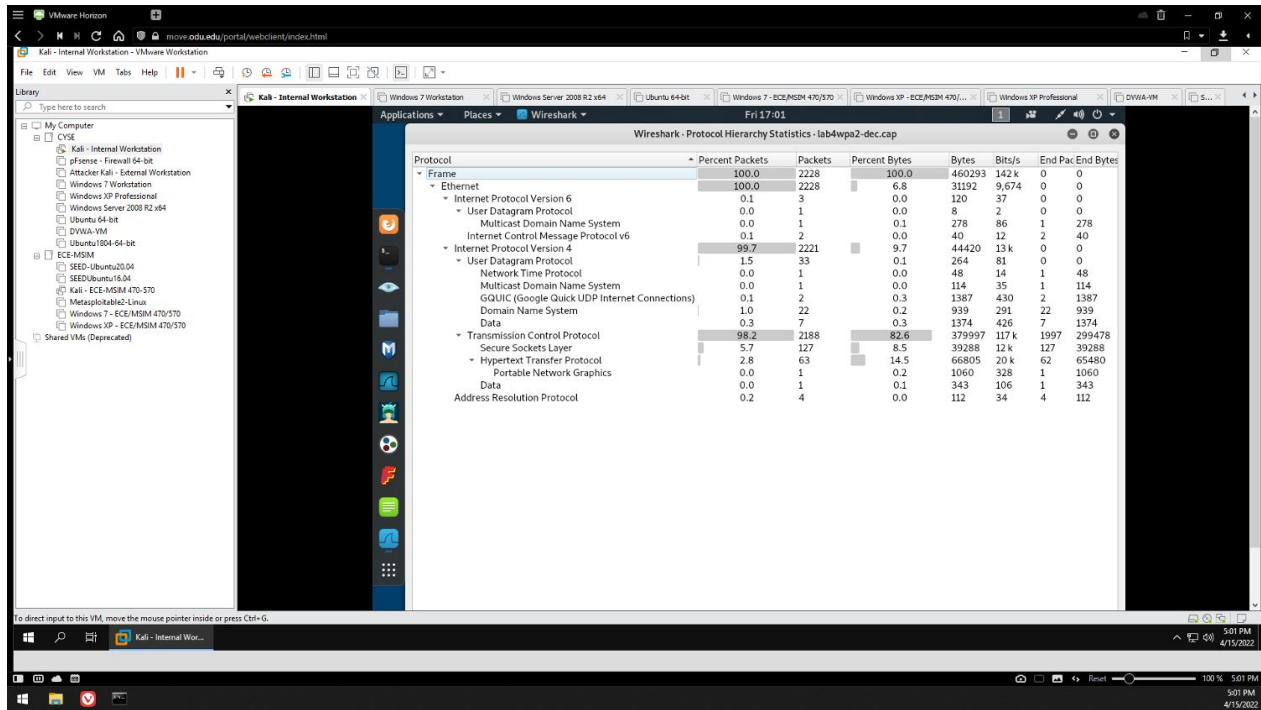
Figure 11 - Wireshark Protocol Hierarchy Statistics of lab4pa2-dec.cap
