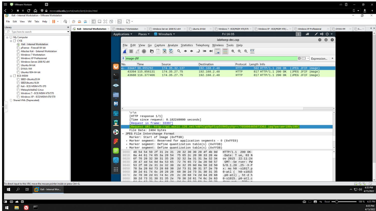
Figure 6 - URI to JPG image found in HTTP packet
