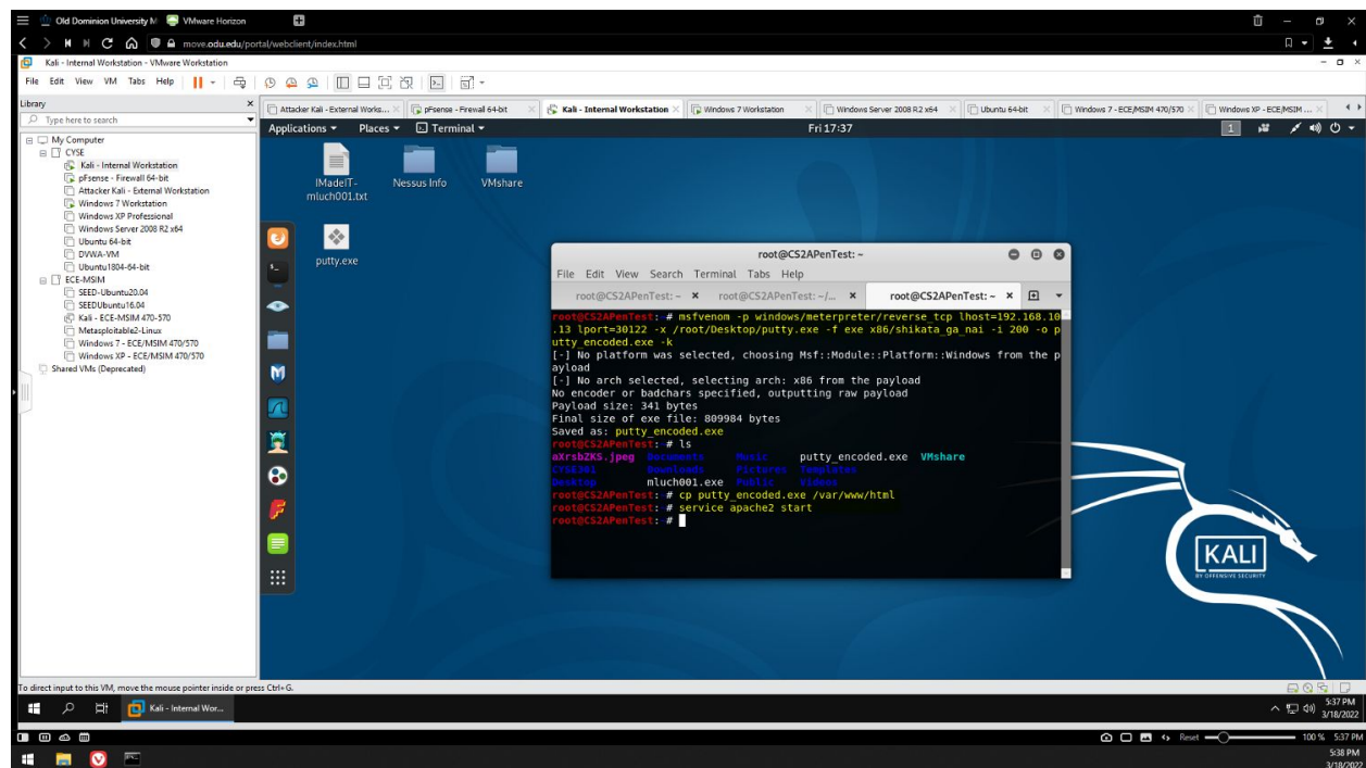
Figure 21 - Injecting encoded payload into putty.exe
