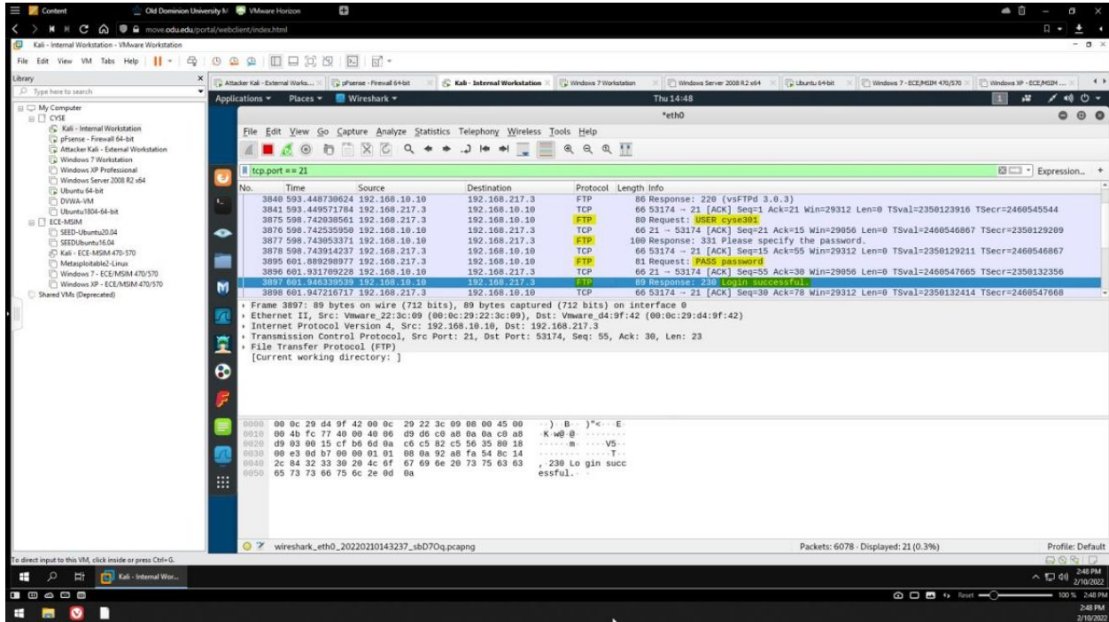
Figure 10 Internal Kali VM - TCP port 21 display filter demonstration
