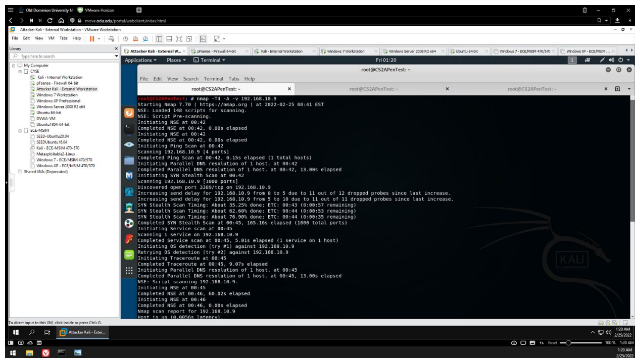
Figure 16 - External Kali intense scan on Windows 7
