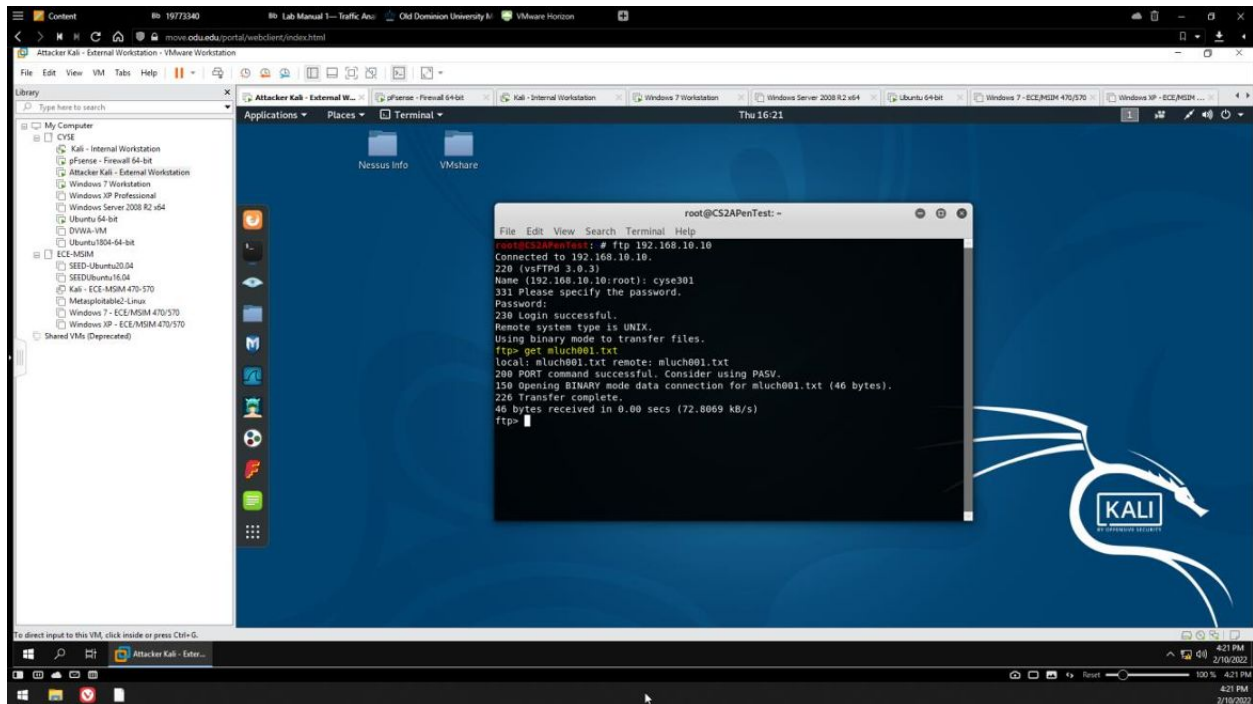
Figure 13 External Kali VM - Transferring mluch001.txt from Ubuntu VM over the FTP server
