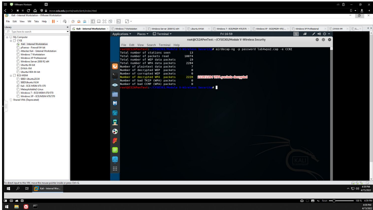
Figure 10 - lab4wpa2.cap 2228 WPA packets decrypted with airdecap-ng
