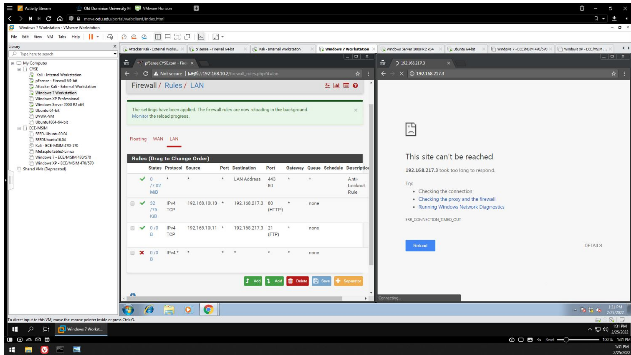
Figure 9 - pfSense firewall ruleset (LAN) to allow only HTTP and FTP from External Kali to Internal Kali and WS 2008 respectively
