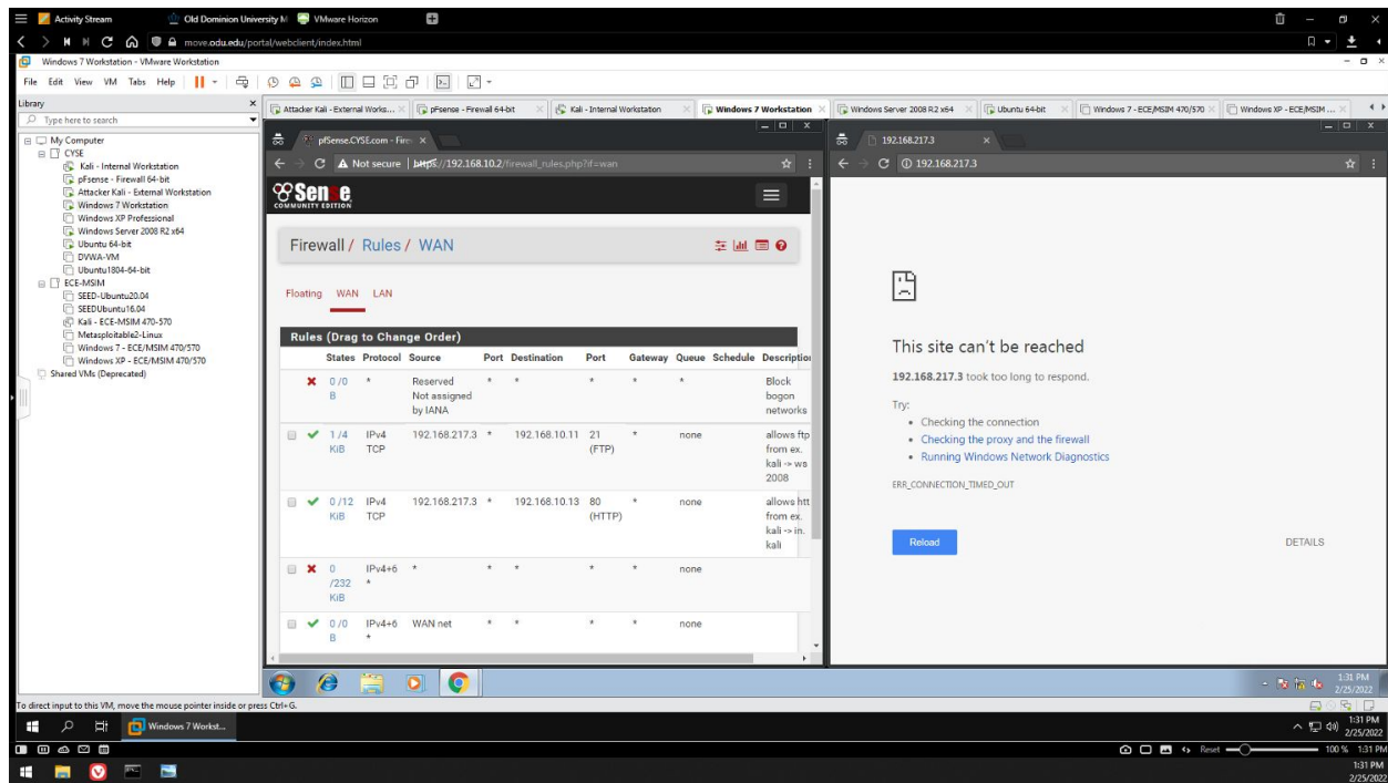
Figure 8 - pfSense firewall ruleset (WAN) to allow only HTTP and FTP from External Kali to Internal Kali and WS 2008 respectively
