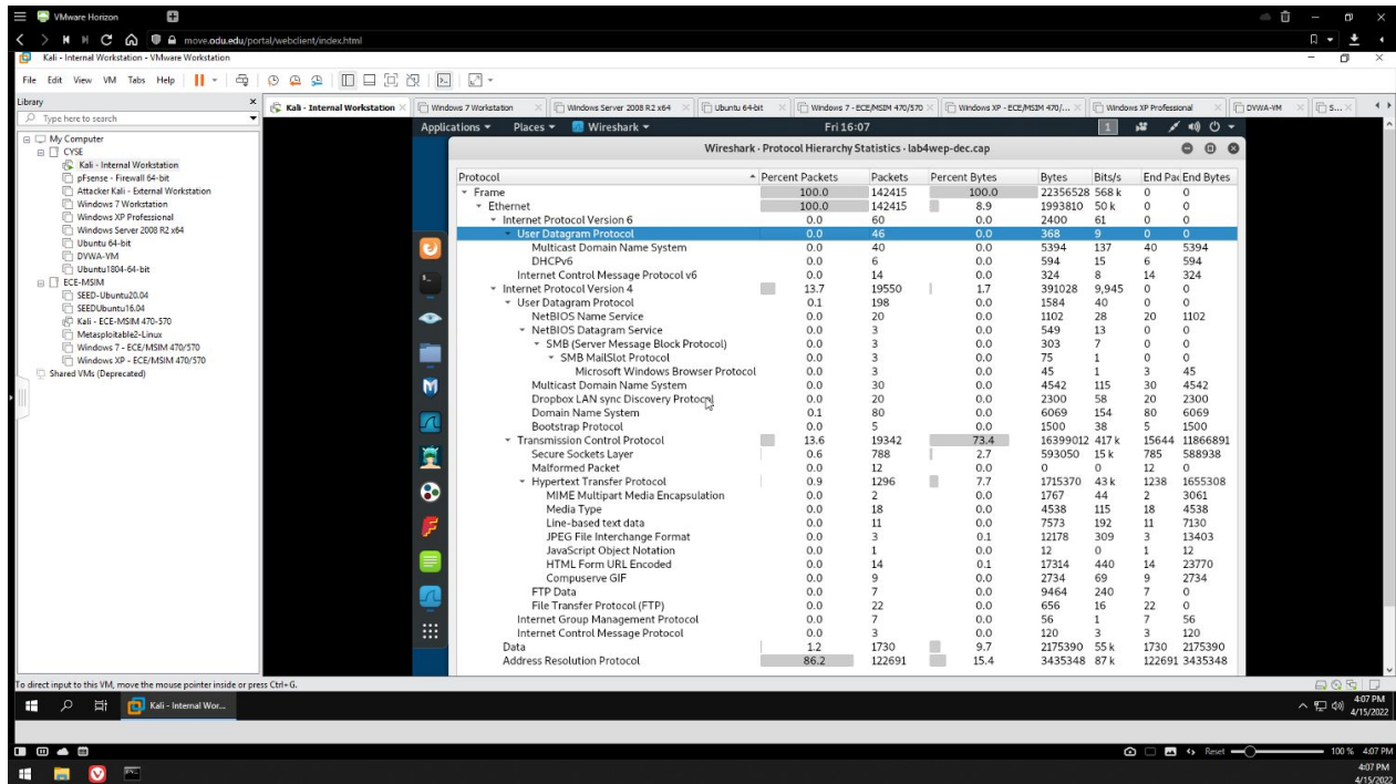
Figure 4 - Wireshark Protocol Hierarchy Statistics of lab4wep-dec.cap
