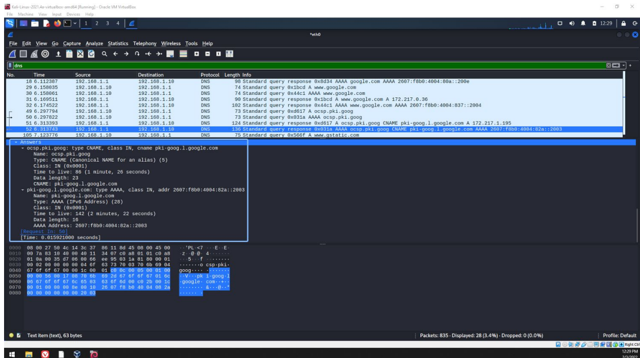
Figure 7 Query answers for second pair
