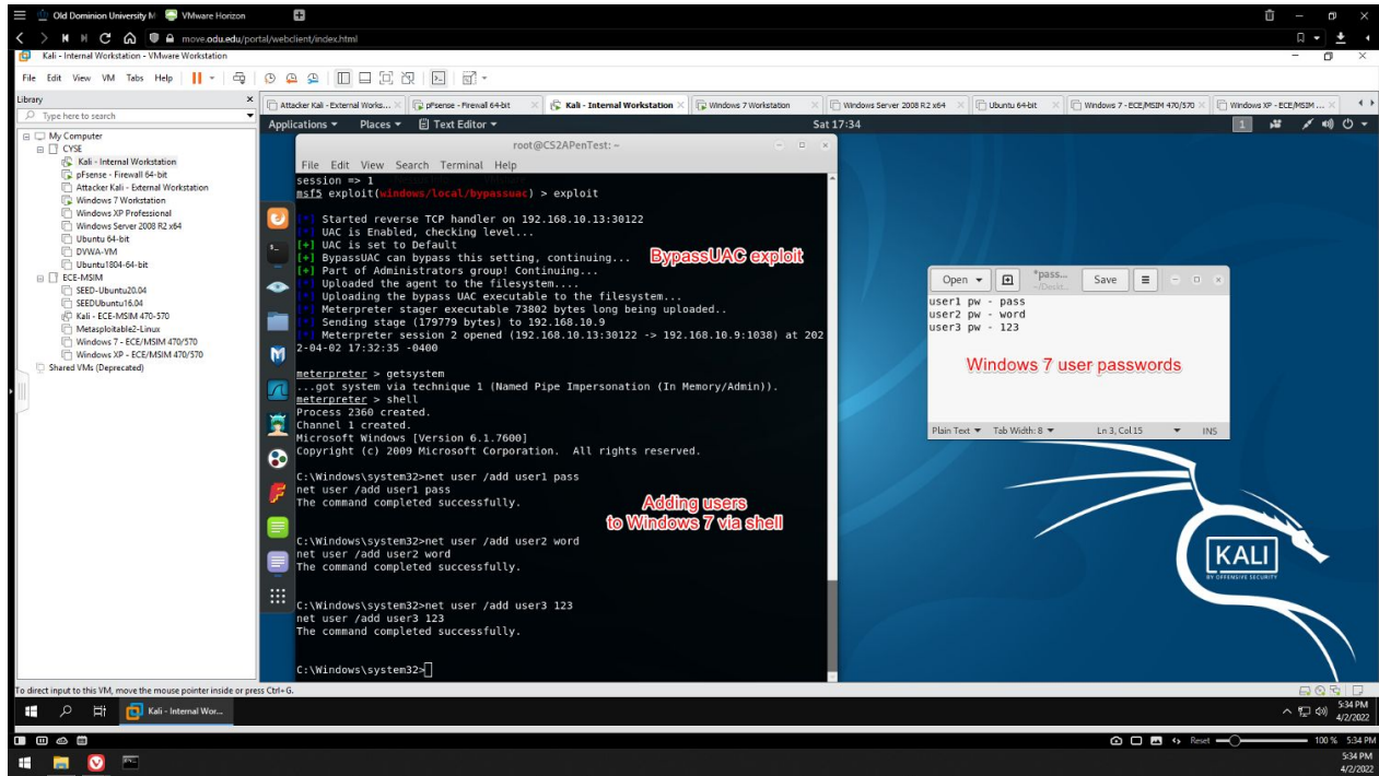
Figure 4 - Using bypassuac exploit to create users on Windows 7 VM
