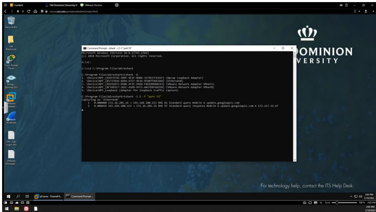
Figure 2 tShark w/ "port 53" capture filter active
