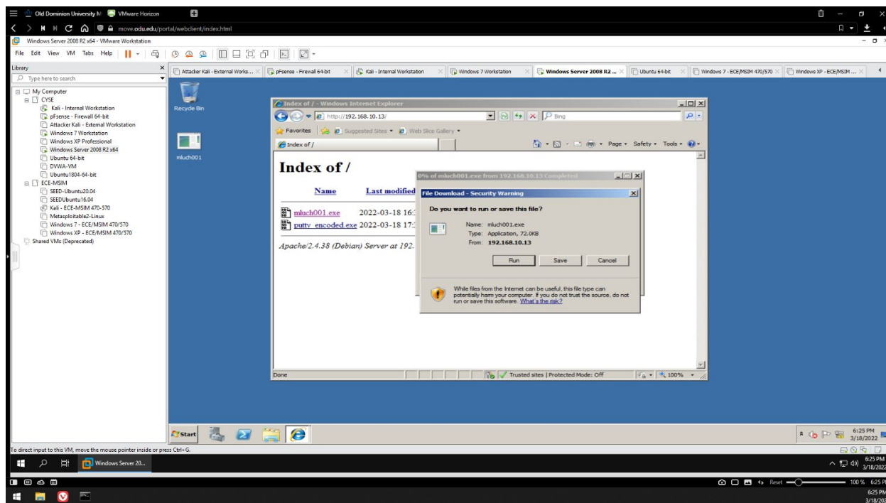
Figure 23 - WS 2008 R2 - Downloading and running reverse tcp payload
