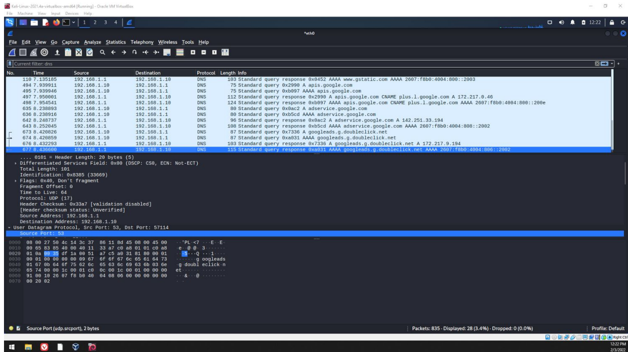
Figure 1 Captured packets displayed in Wireshark
