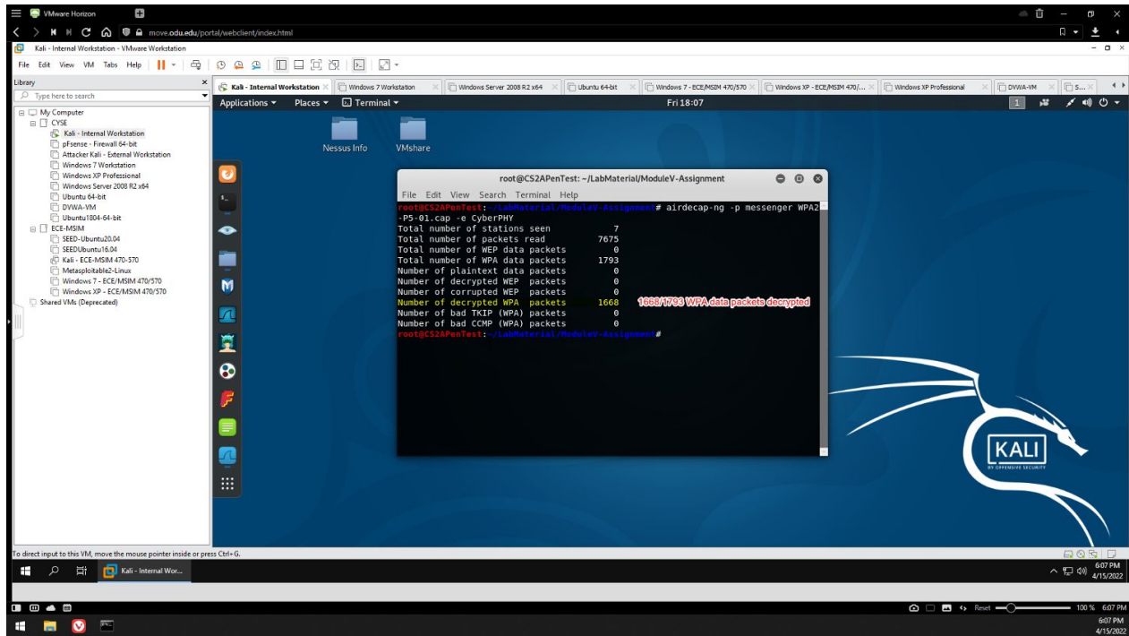
Figure 16 - WPA2-P5-01.cap WPA data packet decryption
