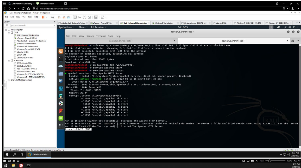
Figure 1 - Creating the payload in msfvenom and hosting it on Apache HTML server
