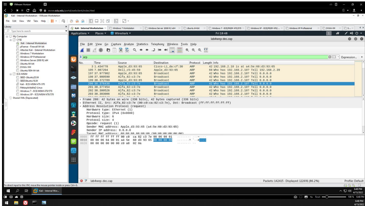
Figure 5 - Abnormal traffic detected (ARP scan)
