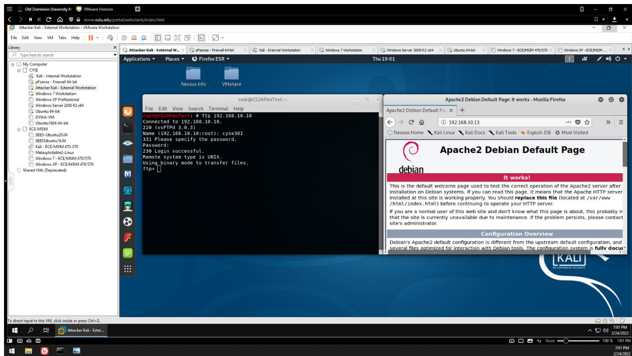
Figure 3 - Accessing Ubuntu via FTP and Internal Kali VM via HTTP from External Kali VM
