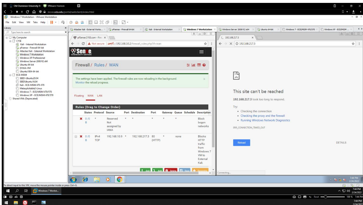
Figure 7 - pfSense ruleset to block HTTP traffic from Windows 7 VM to External Kali VM
