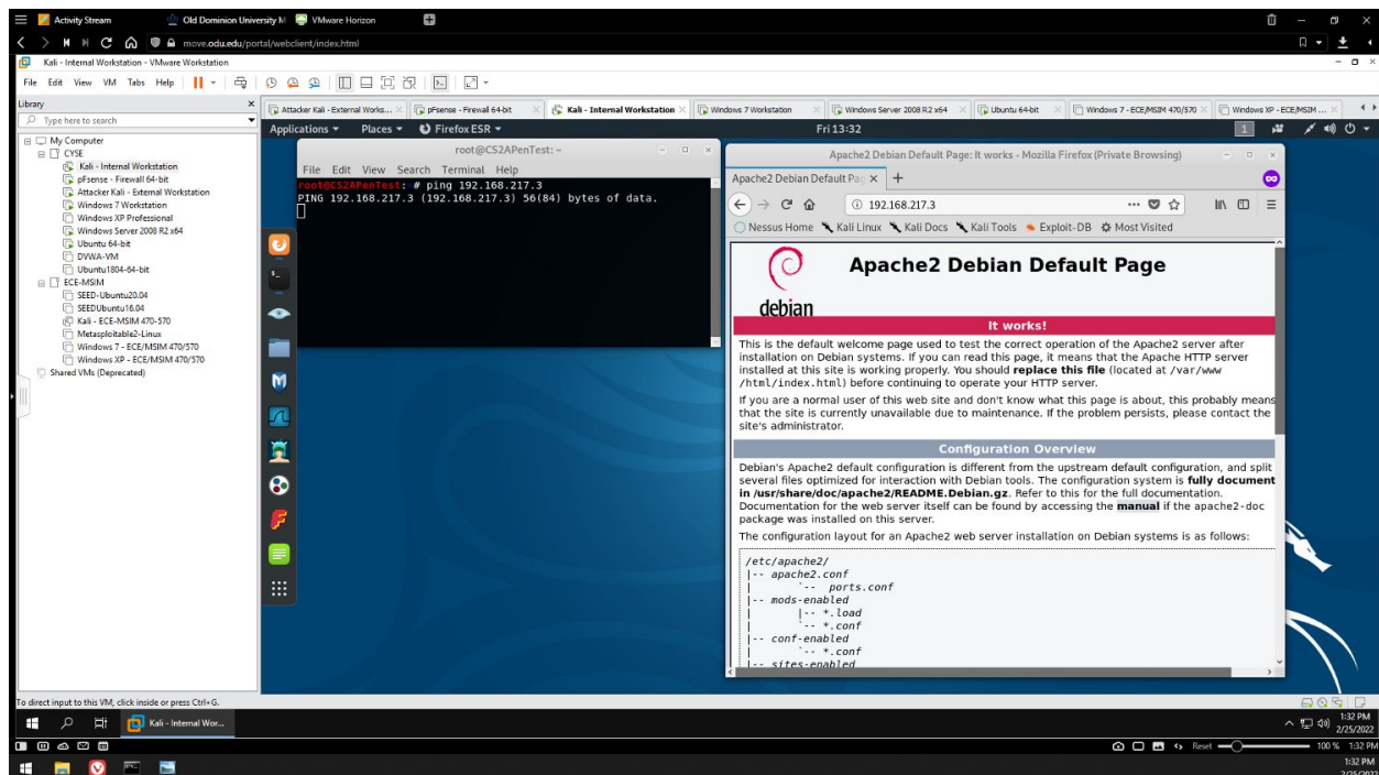
Figure 10 - pfSense firewall ruleset: Testing the ICMP and HTTP connections from Internal Kali to External Kali
