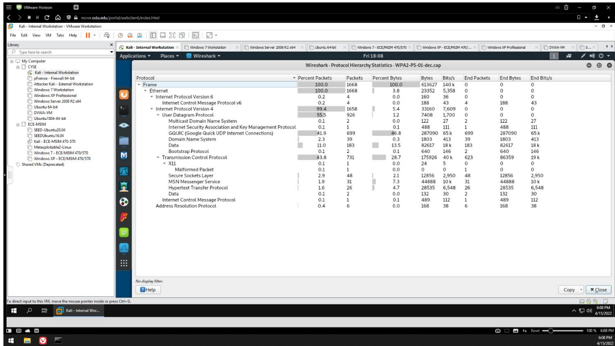
Figure 17 - Wireshark Protocol Hierarchy Statistics of WPA2-P5-01-dec.cap
