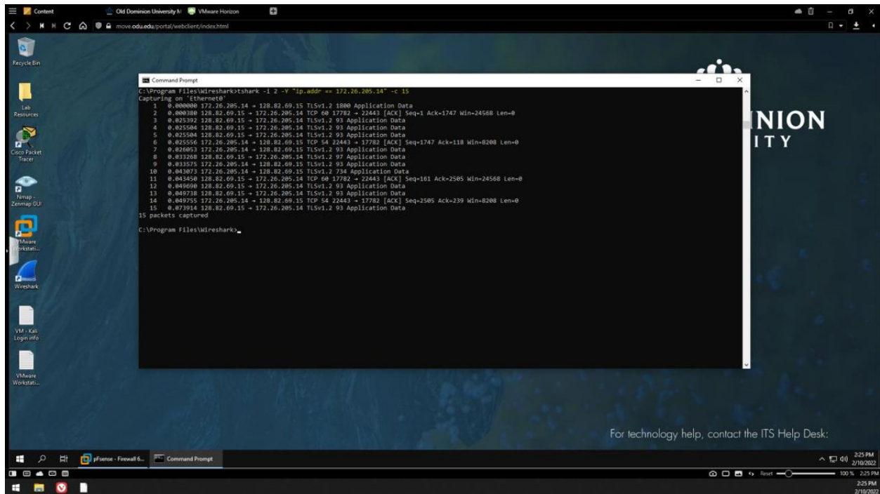
Figure 6 tShark IP address display filter demonstration
