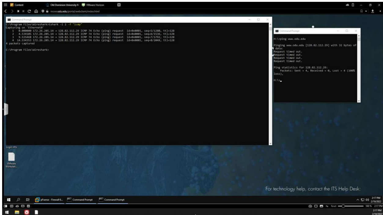
Figure 4 Captured ICMP packets displayed in tShark
