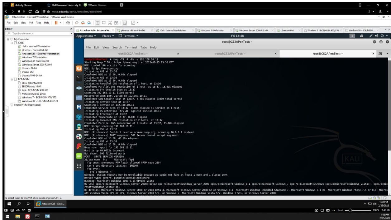
Figure 21 - External Kali intense scan on WS 2008 (with firewall ruleset applied)
