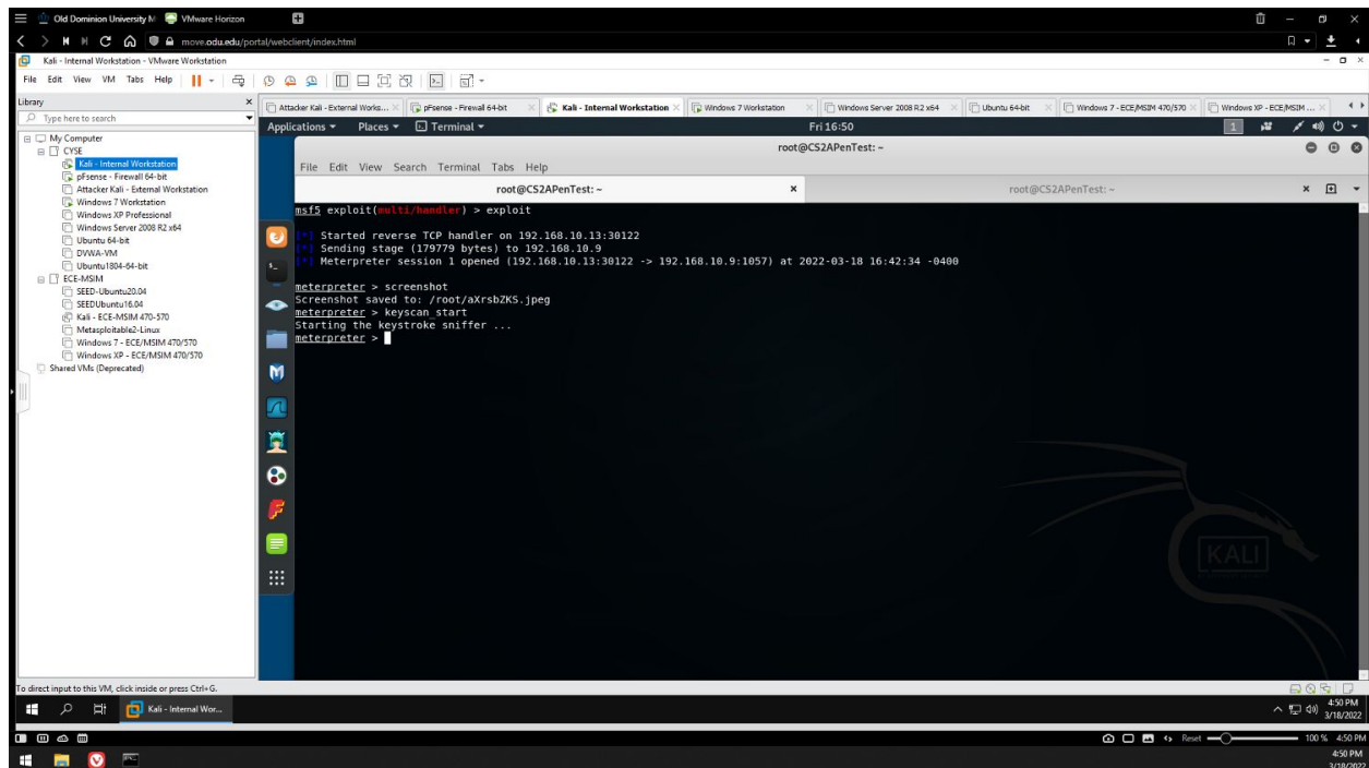
Figure 6 - Starting the keystroke sniffer
