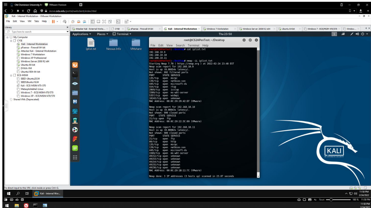
Figure 12 - Internal Kali simple Nmap scan 192.168.10.9-192.168.10.11
