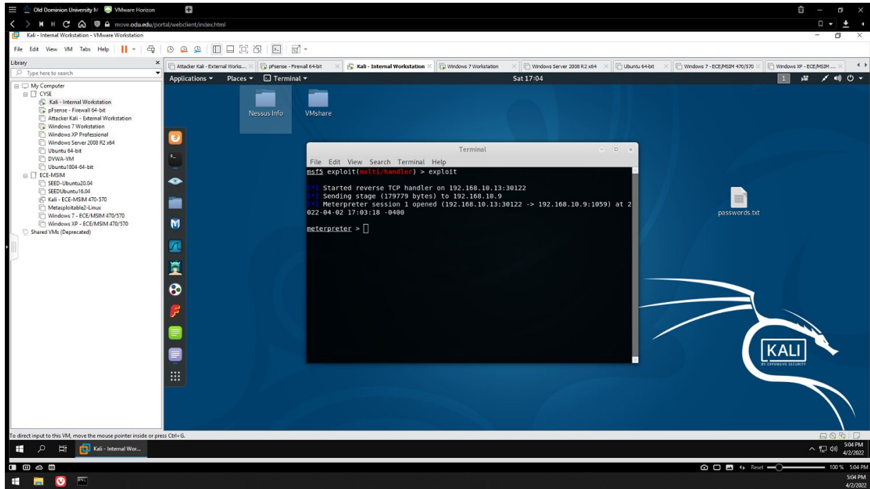
Figure 3 - Starting reverse shell connection to Windows 7 VM
