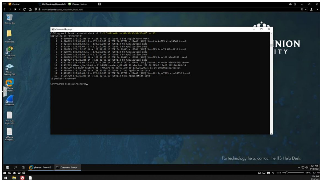
Figure 5 tShark MAC address display filter demonstration
