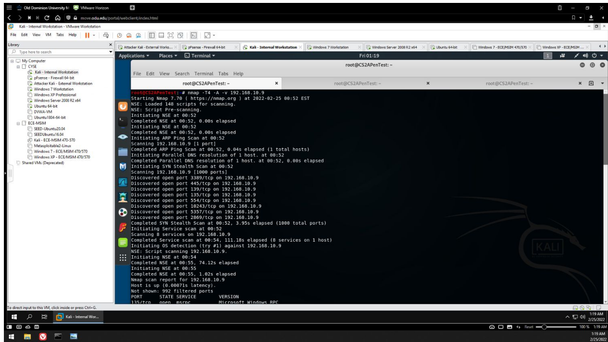
Figure 13 - Internal Kali intense scan on Windows 7
